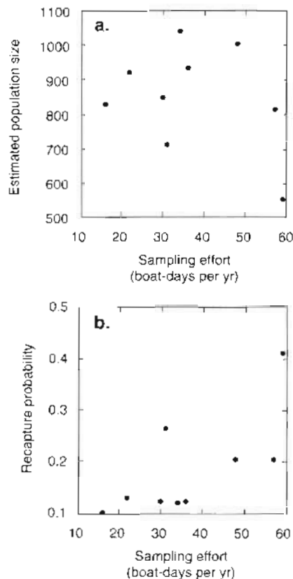
Fig. 3. Megaptera novaeangliae . Relationship between annual sampling effort in Hervey Bay (boat days yr -1 ) and (a) estimated annual EAGVS humpback abundance in Hervey Bay (1988 to 1996, Table 1) and (b) estimated resight or recapture probability (1988 to 1996) derived from Model B (constant survival, time-varying resight)
